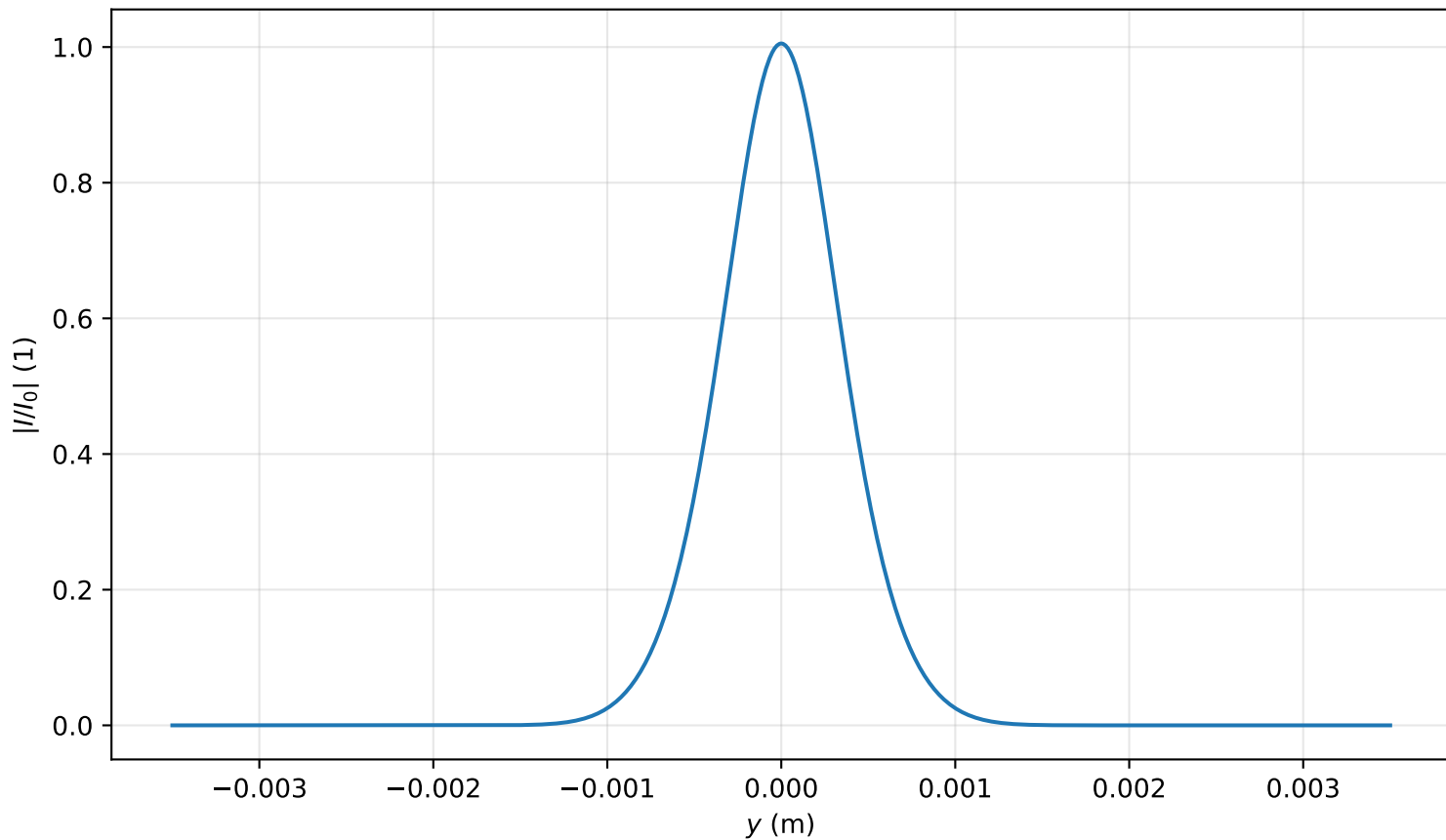
Intensity profile I(x=0, y, z=0.876)/I_0 , P_{in}=0.4P_{cr} , artificial time
